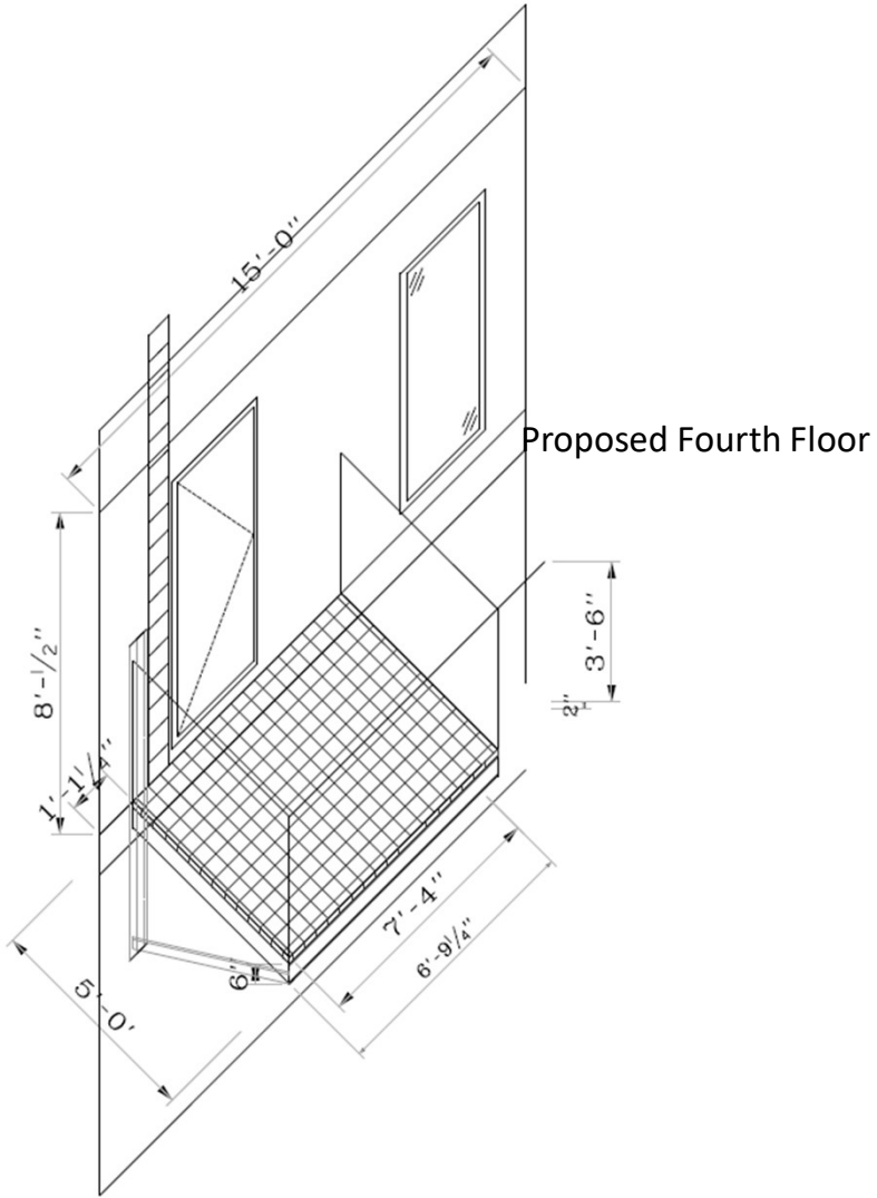
Proposed 3D Rear view of 404A Henry Street
