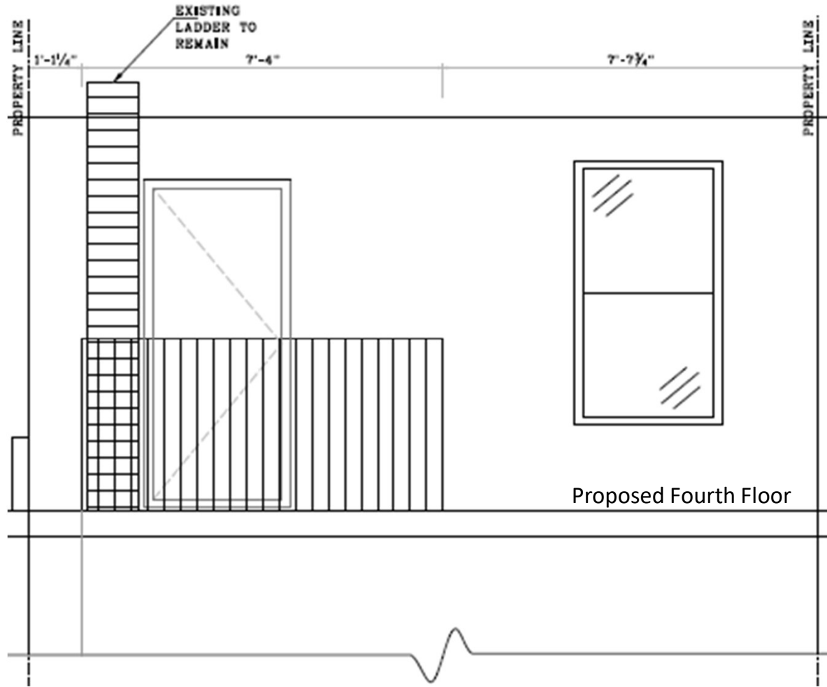
Proposed Rear Elevation of 404A Henry Street
