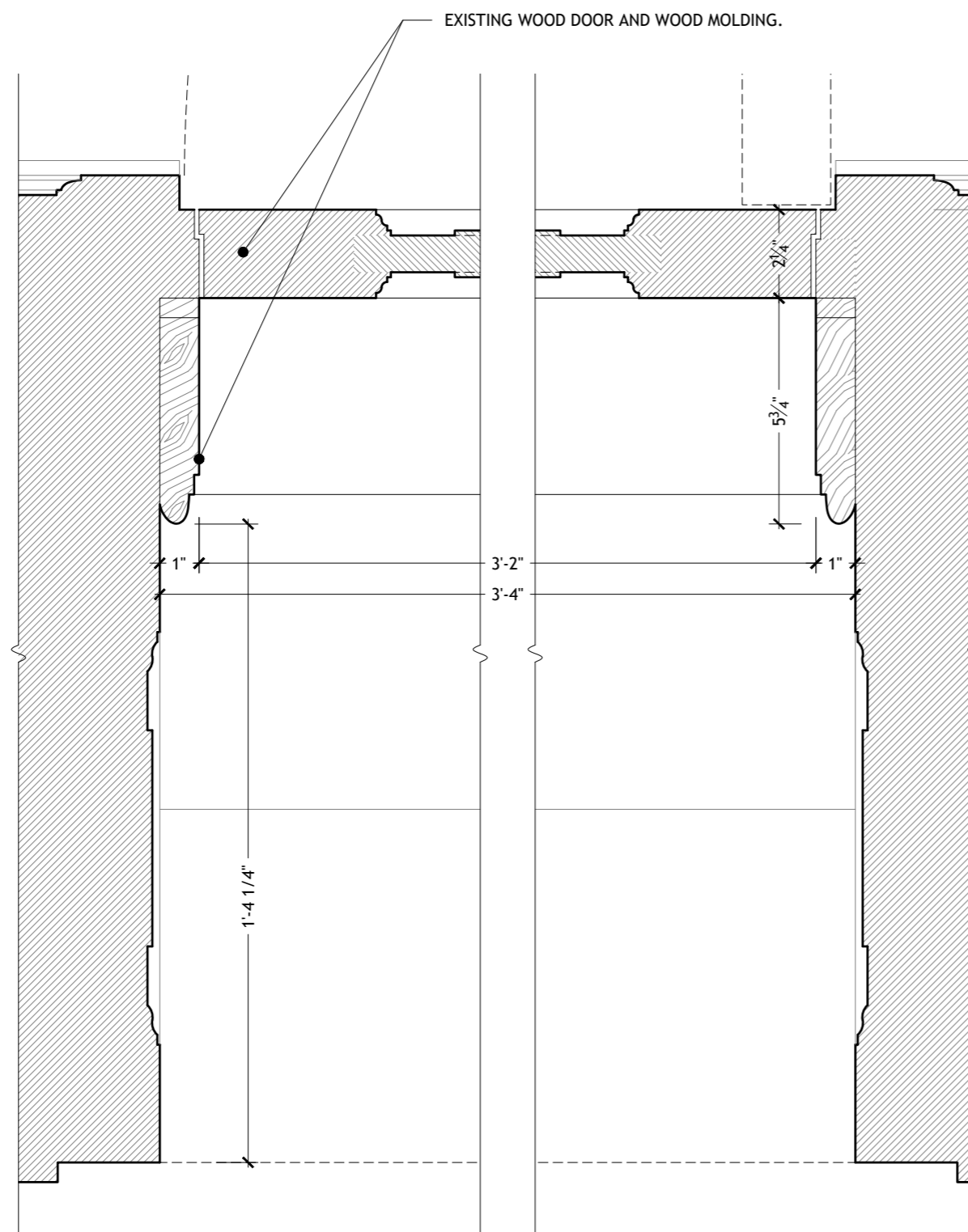
EXISTING
