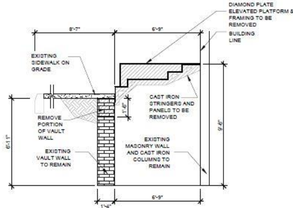
1 EXISTING VAULT SECTION
