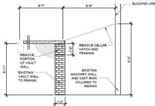
3 EXISTING VAULT HATCH SECTION
