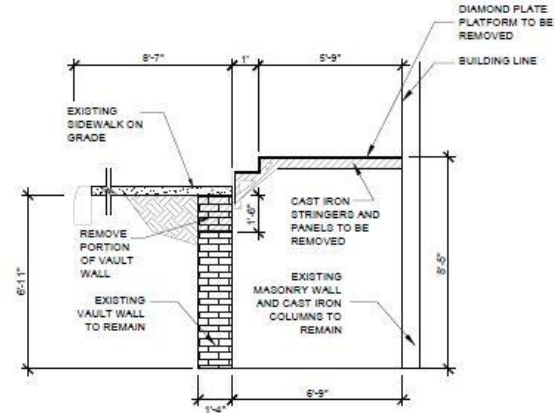
2 EXISTING VAULT SECTION
