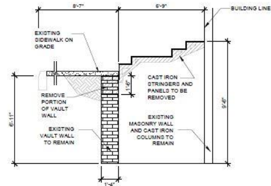
4 EXISTING VAULT SECTION
