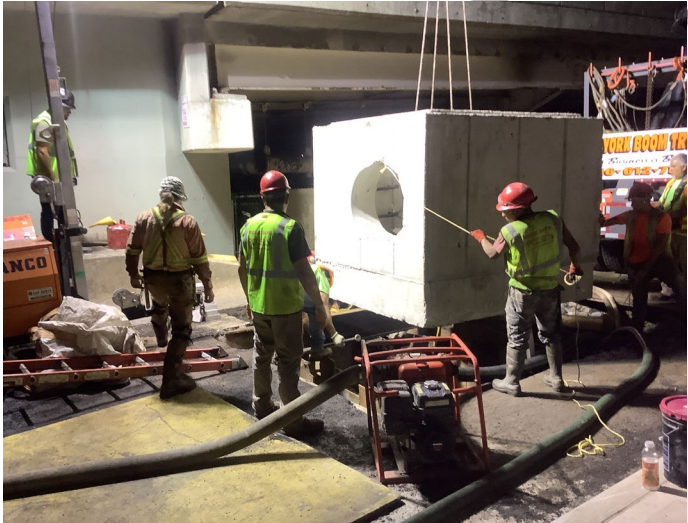
New sewer manholes installed on West Service Rd. – August 2024
