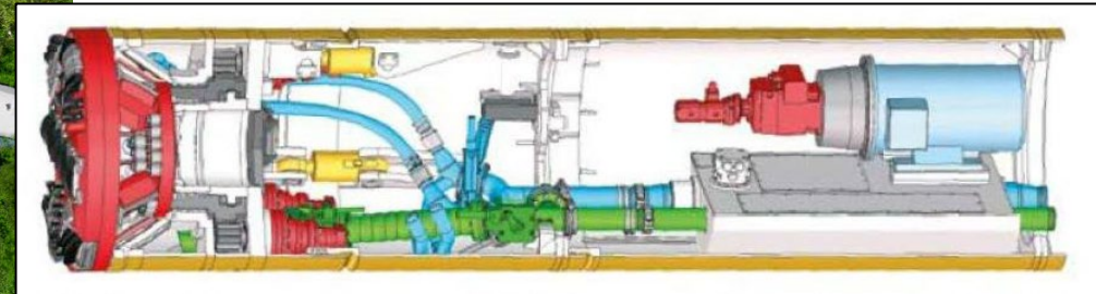
Drawing of microtunneling machine to be used
