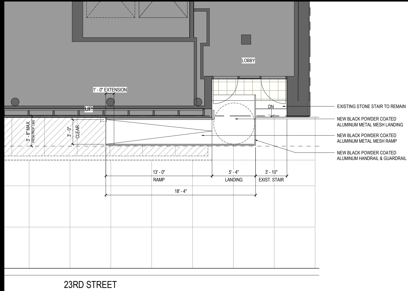
PROPOSED RAMP PLAN AT 23RD STREET
