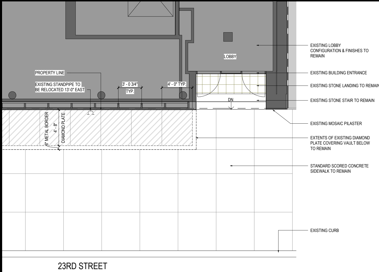
EXISTING PARTIAL PLAN AT 23RD STREET
