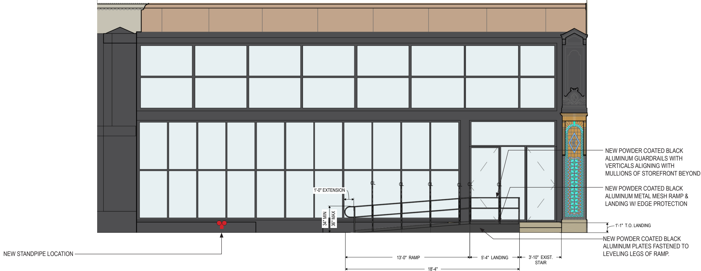
PROPOSED RAMP ELEVATION
