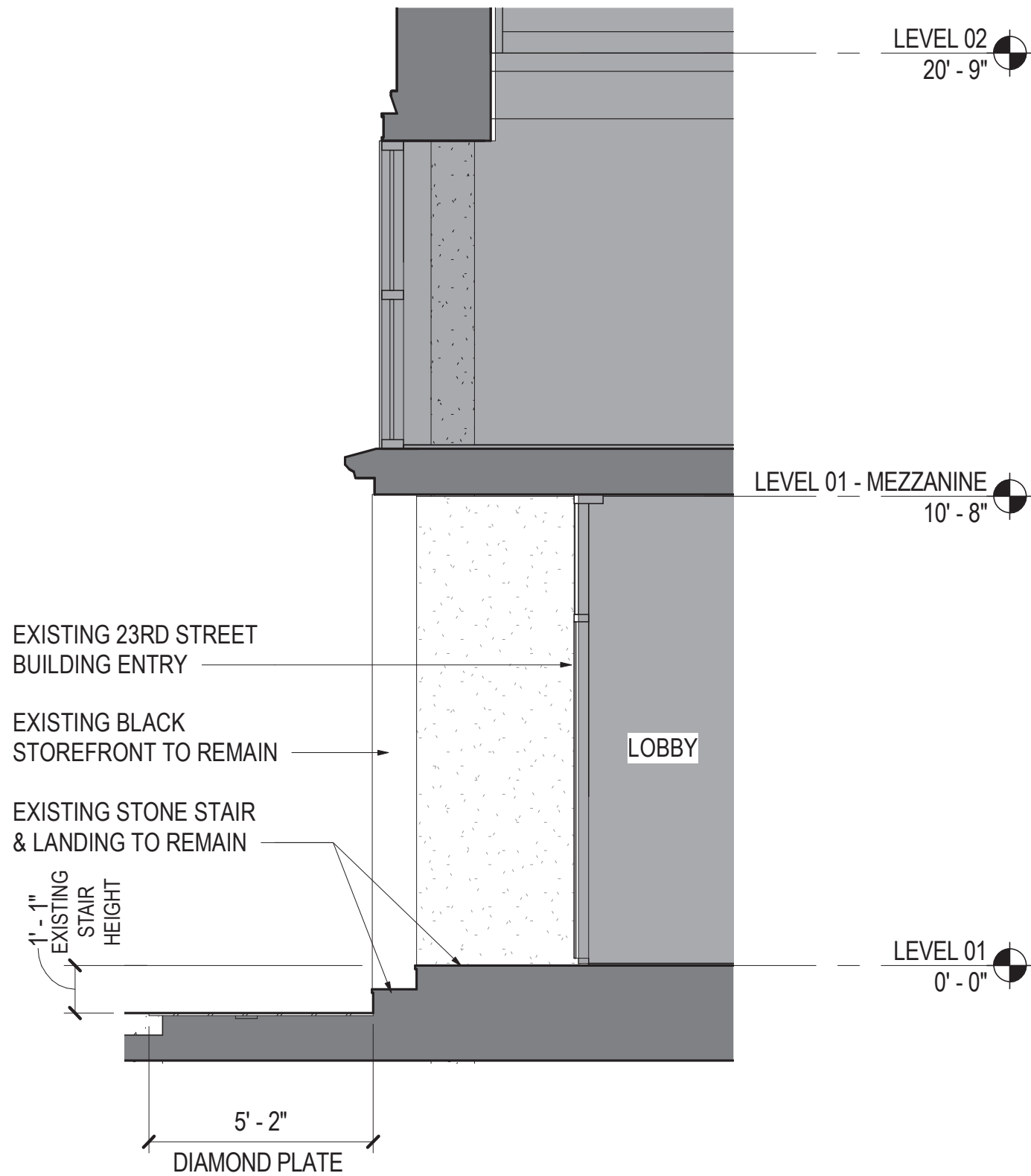
EXISTING FACADE SECTION
