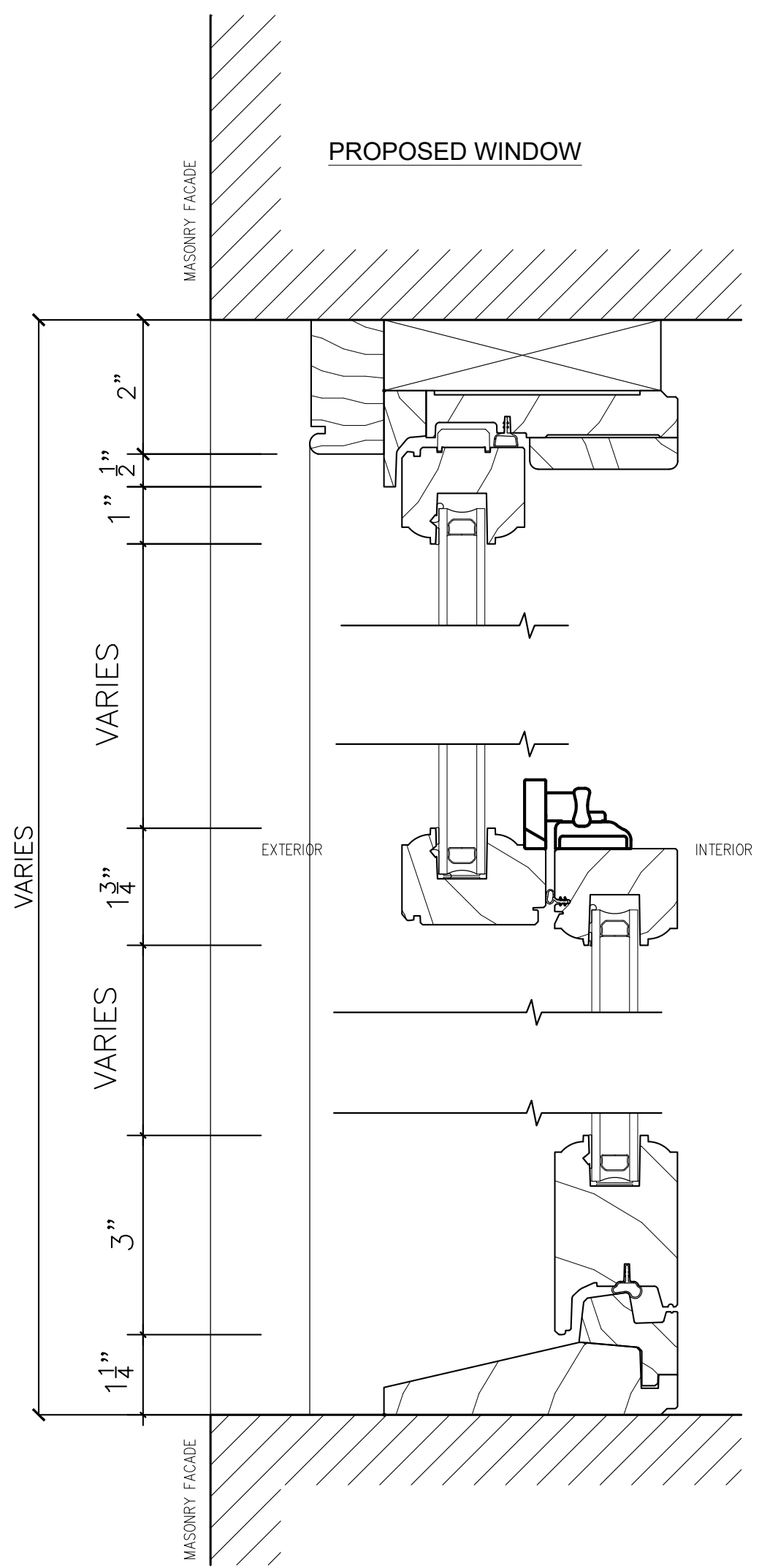
PROPOSED WINDOW SILL AND HEAD DETAILS
