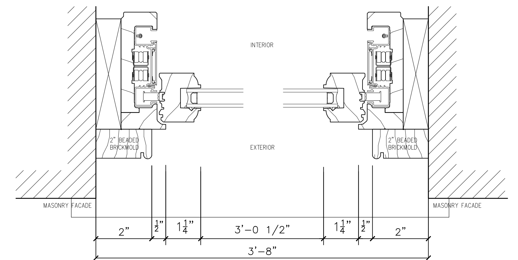
EXISTING WINDOW JAMB DETAILS
