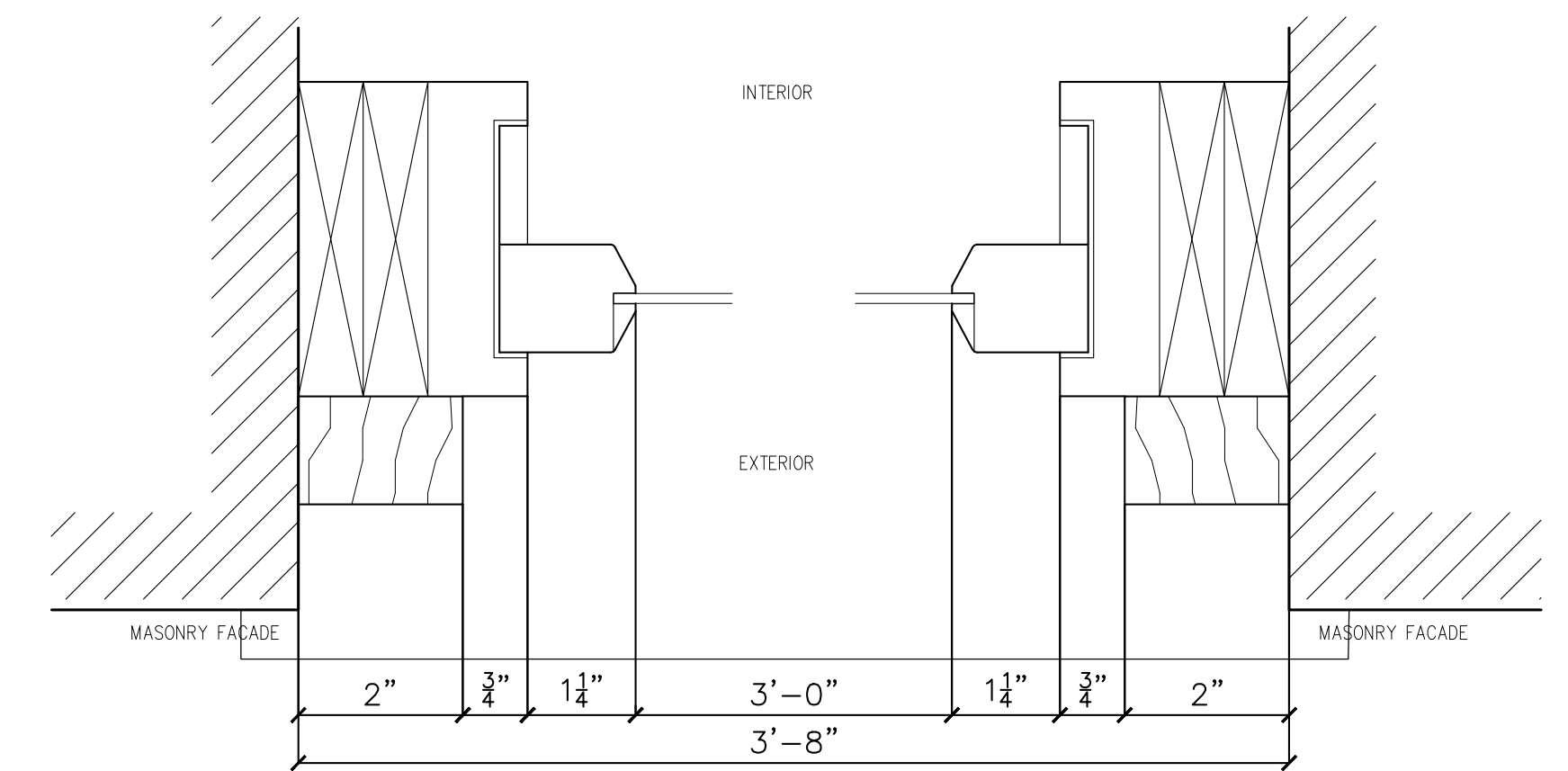
EXISTING WINDOW JAMB DETAILS
