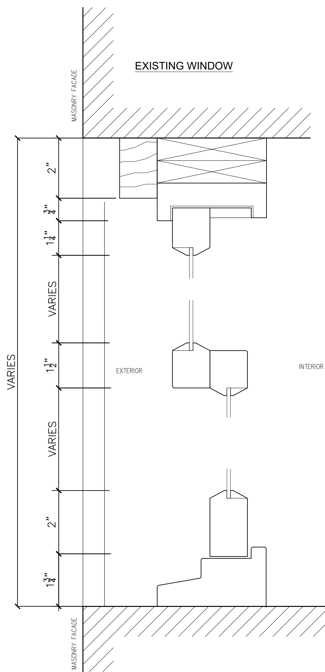
EXISTING WINDOW SILL AND HEAD DETAILS
