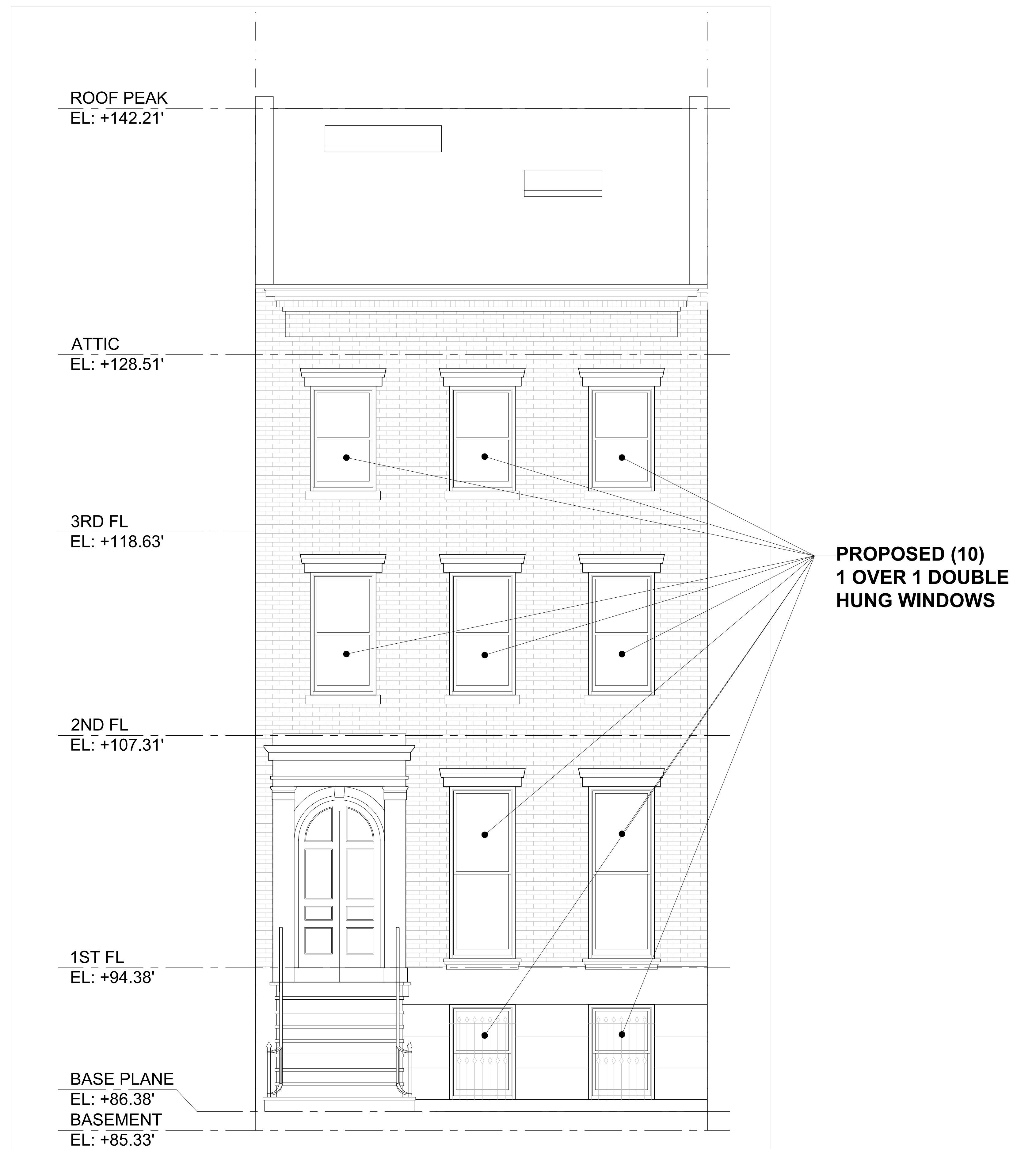
PROPOSED ELEVATION
