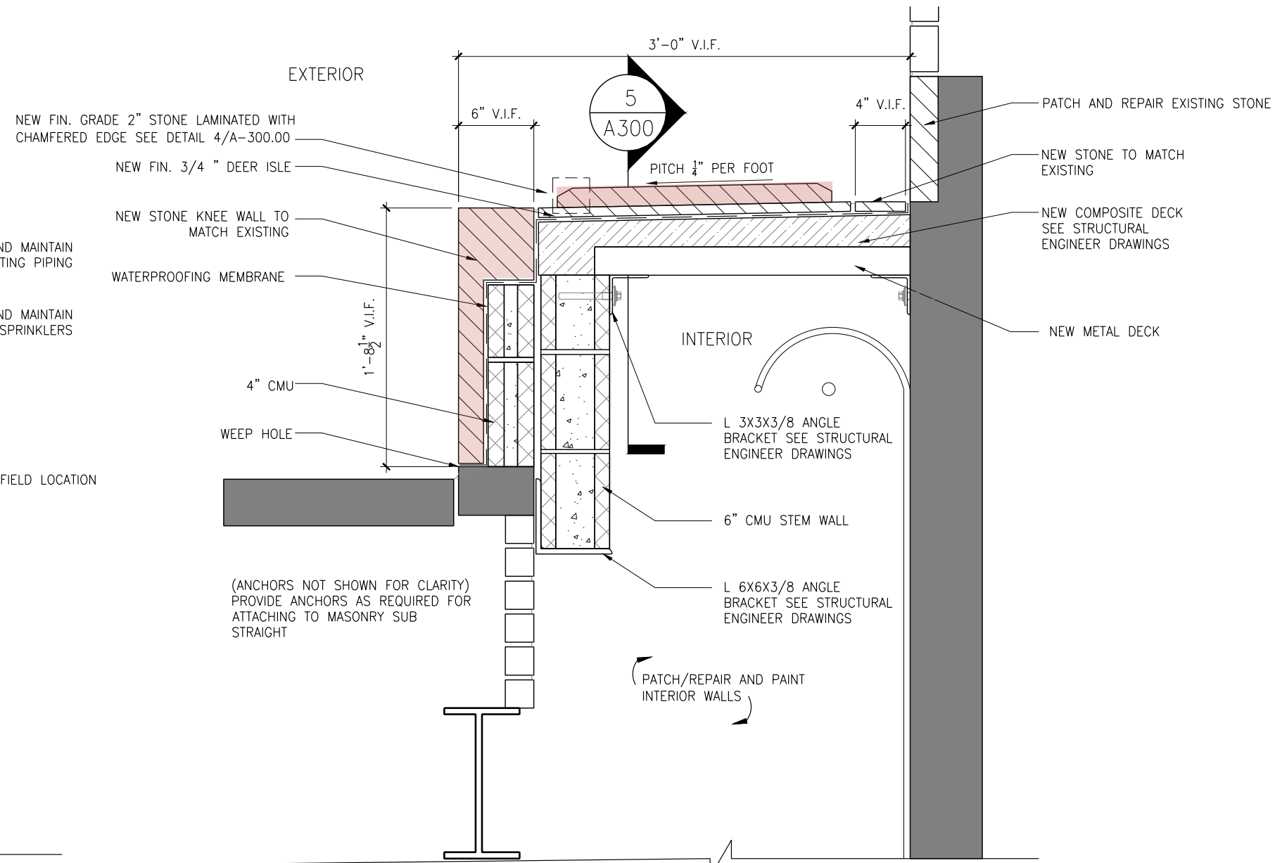
Typ. Proposed Section
