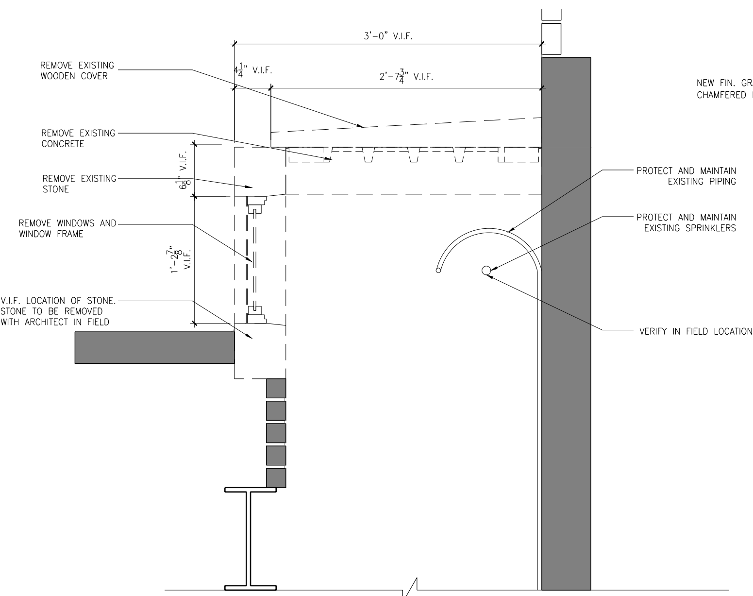
Typ. Demo Section
