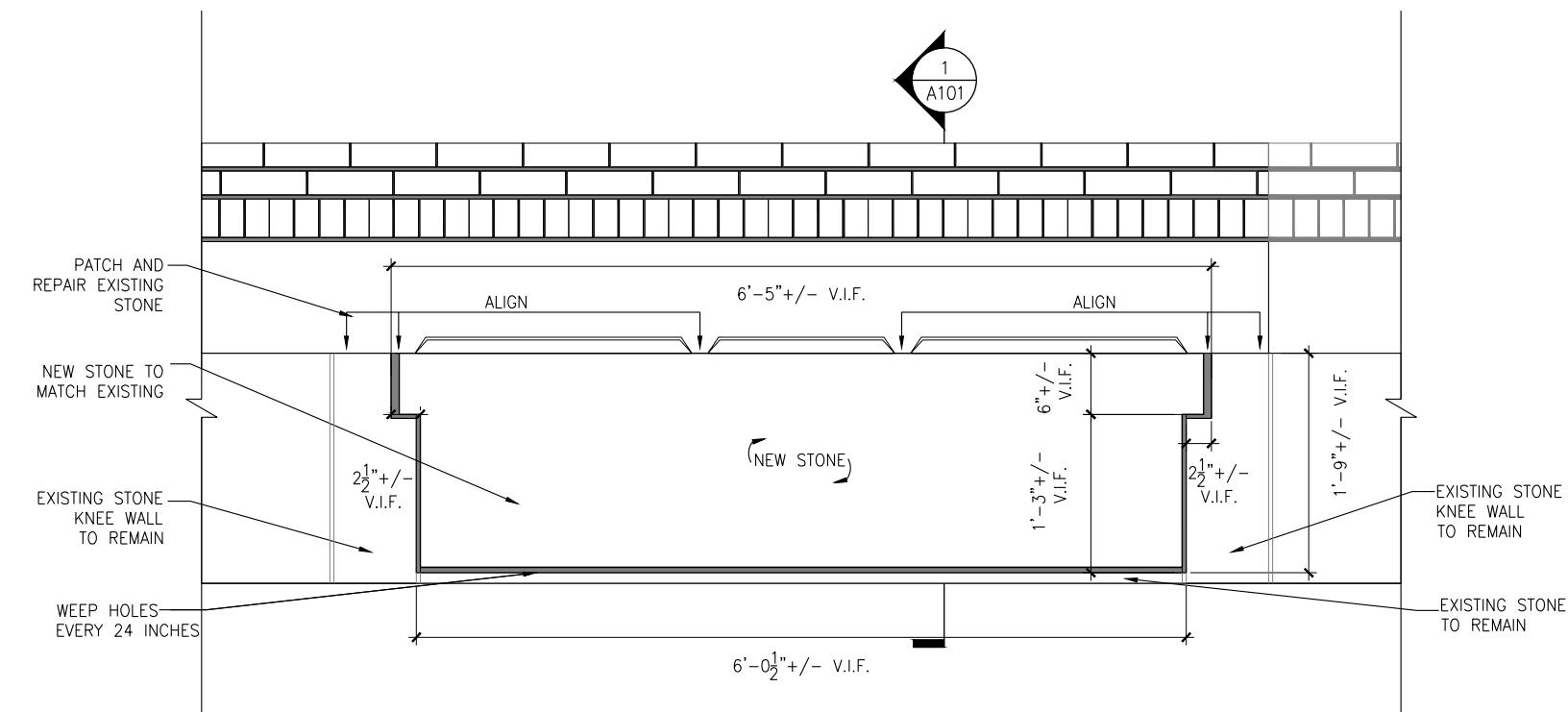
Typ. Proposed Section
