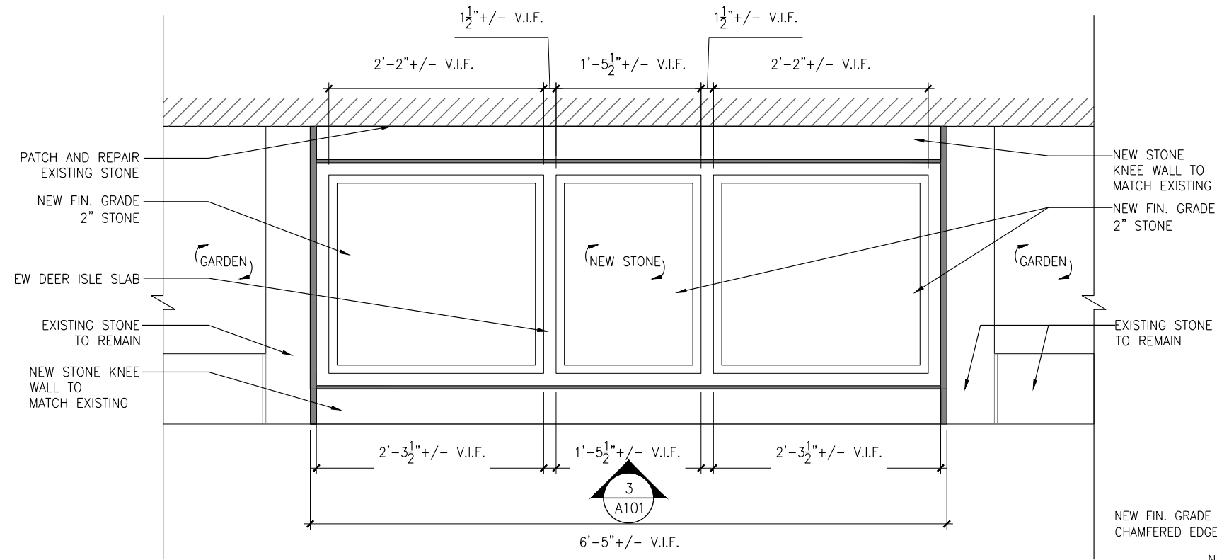
Typ. Proposed Elevation
