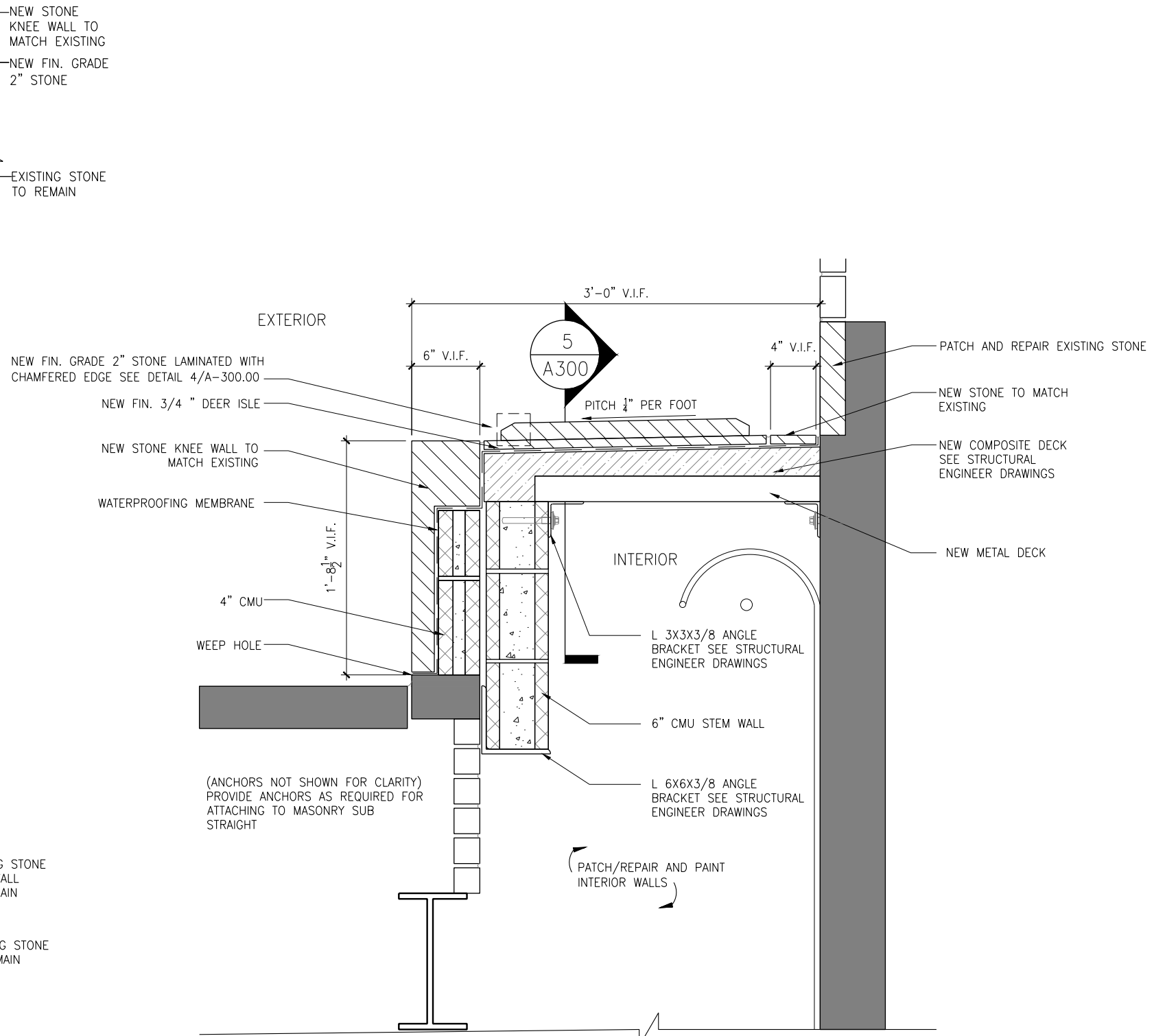
Typ. Proposed Section
