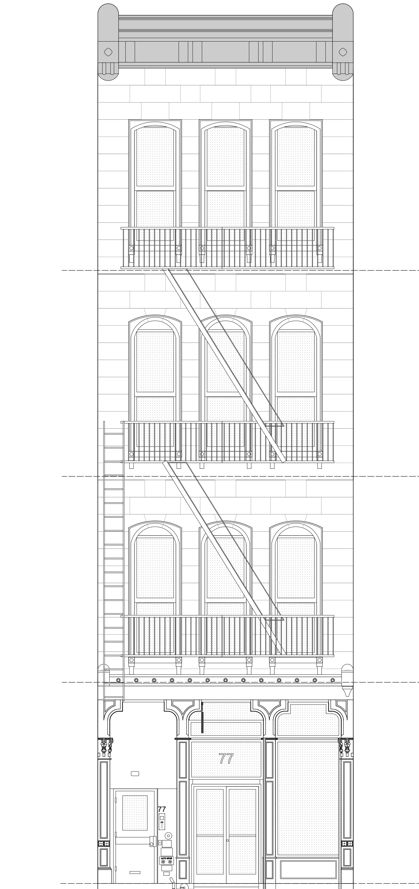
Franklin Street Elevation Prior Condition
