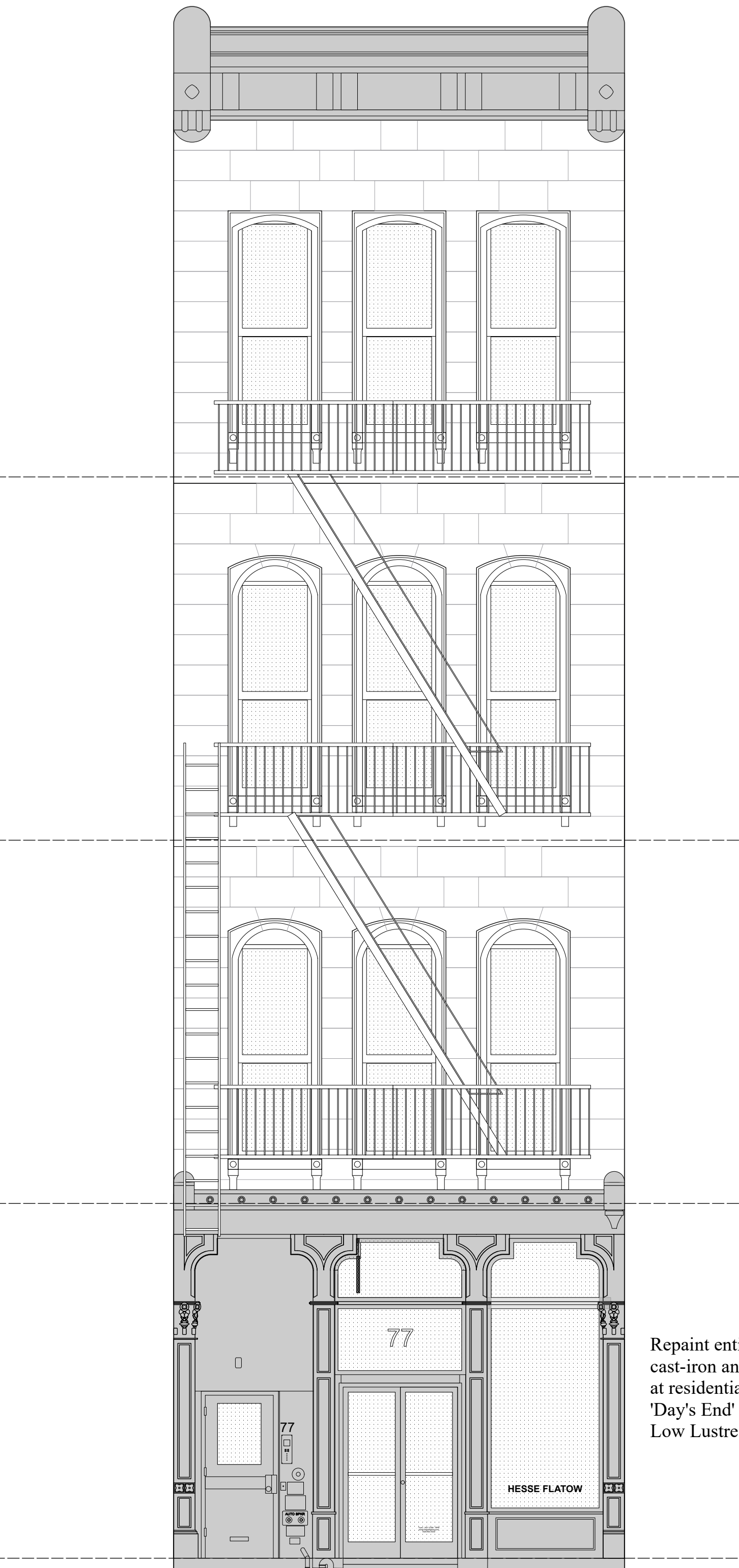
Franklin Street Elevation Proposed Condition
