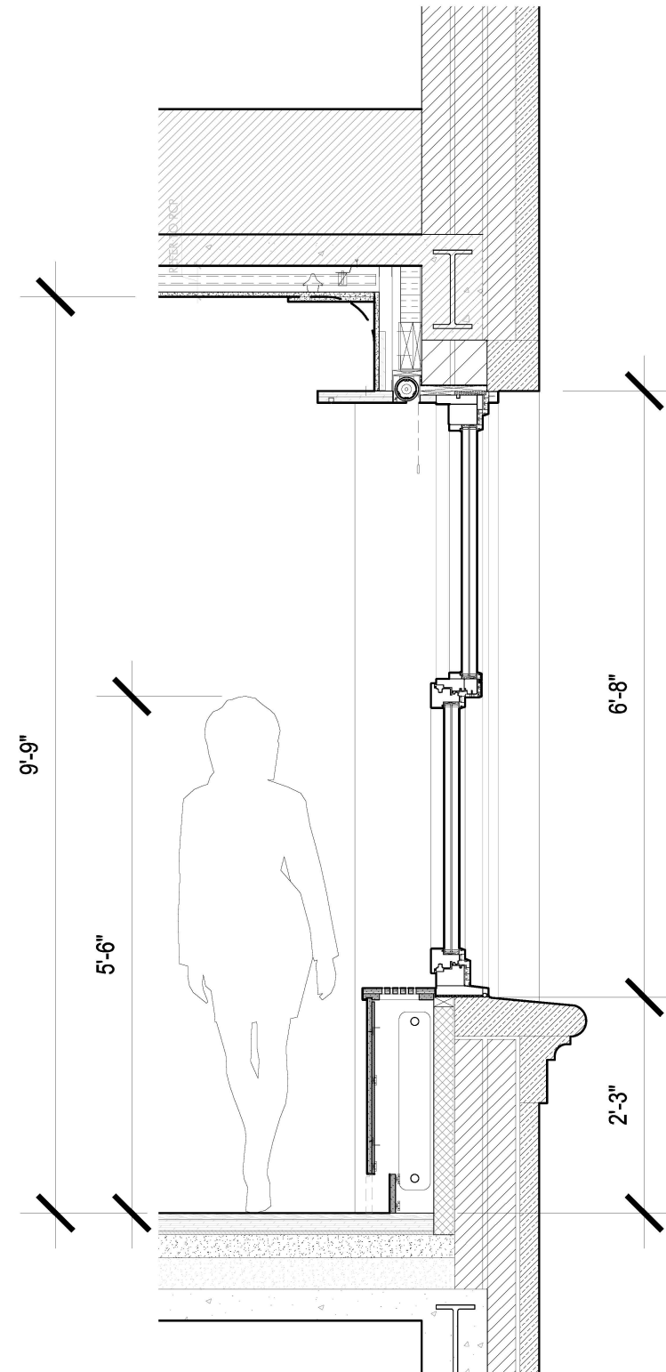
PROPOSED: FULL HEIGHT SECTION DETAIL OF TYP. SIMULATED DOUBLE-HUNG WINDOW
