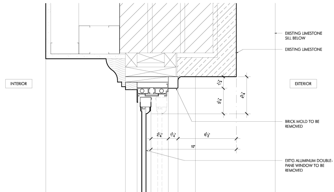
EXISTING: PLAN DETAIL OF TYPICAL ALUMINUM REPLACEMENT DOUBLE HUNG WINDOW @ LOWER LITE
