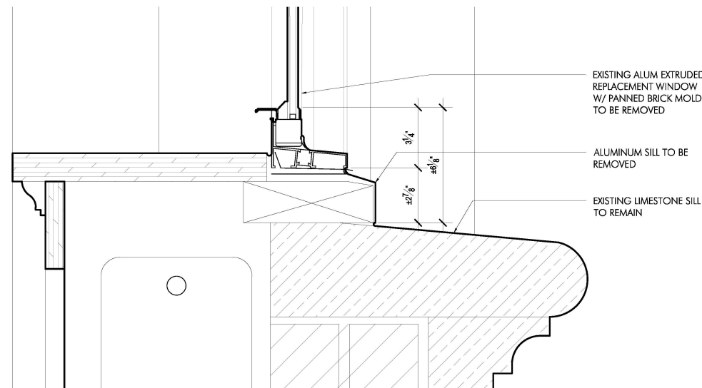
EXISTING: SECTION DETAIL OF TYPICAL ALUMINUM REPLACEMENT DOUBLE HUNG WINDOW
