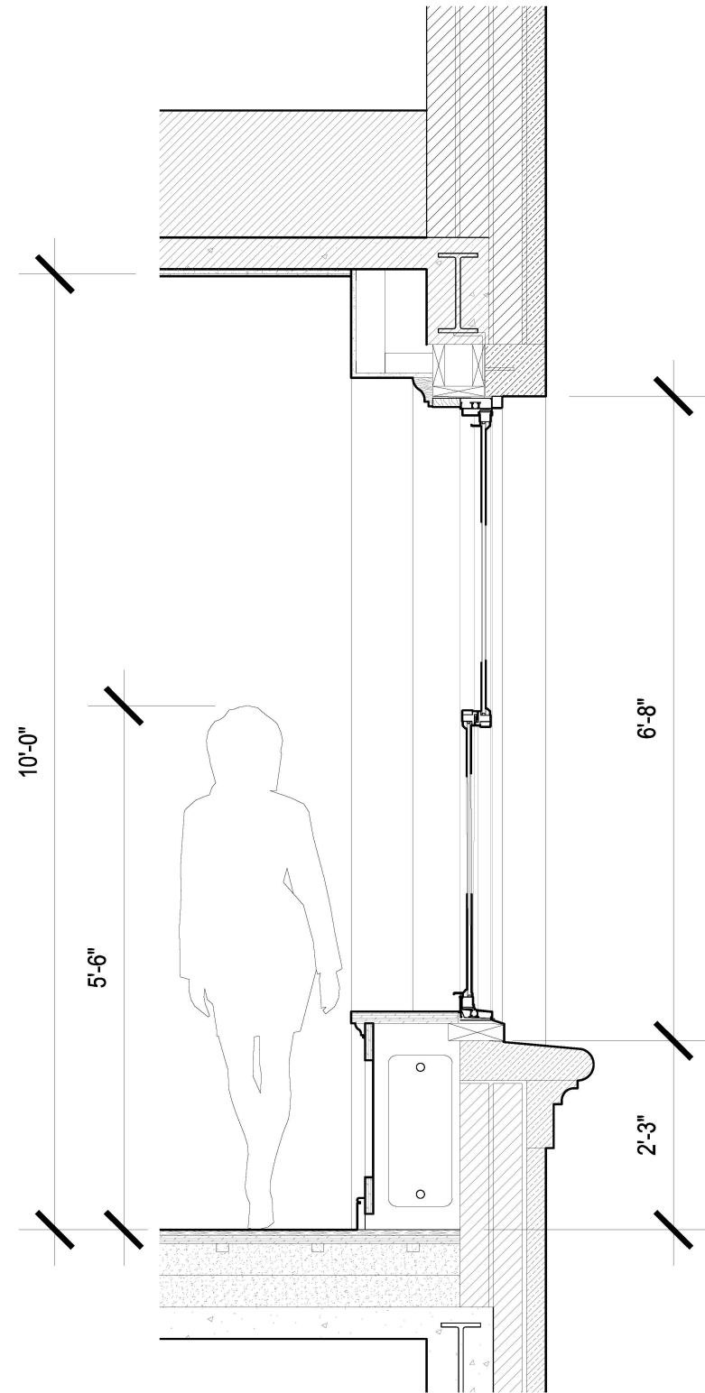
EXISTING: FULL HEIGHT SECTION DETAIL OF TYP. ALUMINUM REPLACEMENT DOUBLE-HUNG WINDOW
