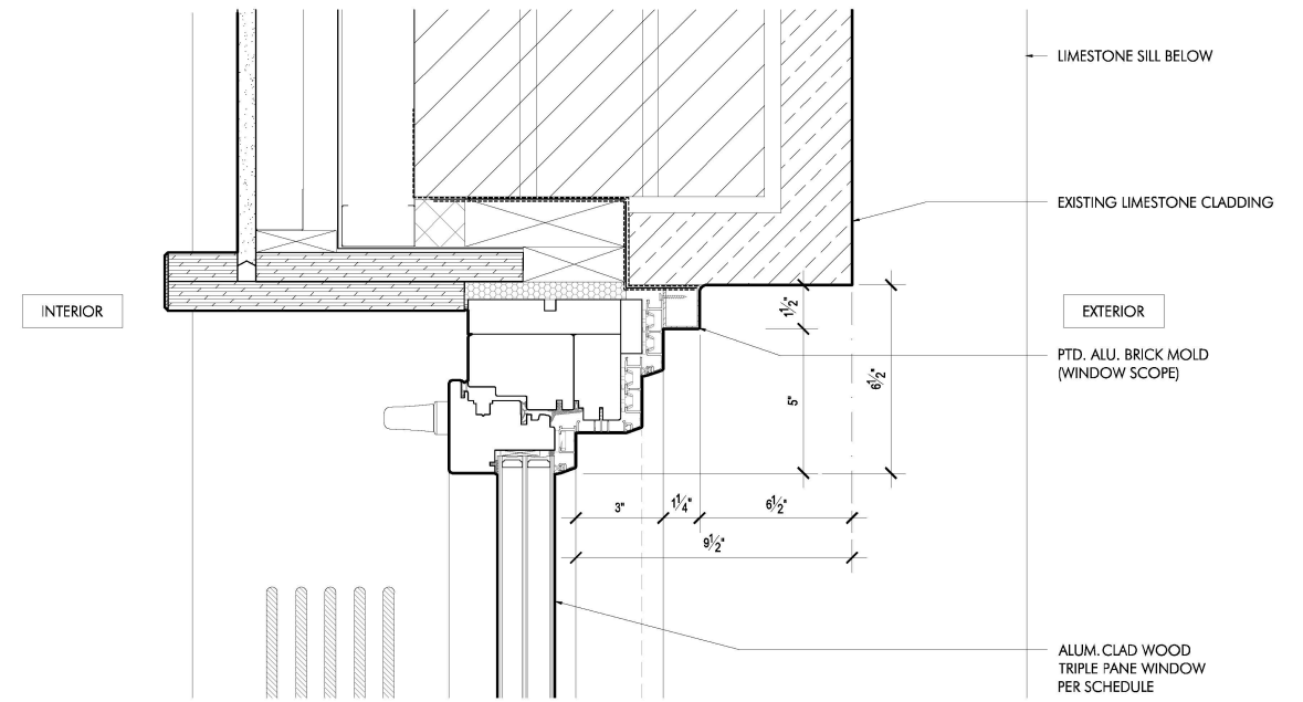
PROPOSED: PLAN DETAIL OF TYPICAL SIMULATED DOUBLE HUNG WINDOW @ LOWER LITE
