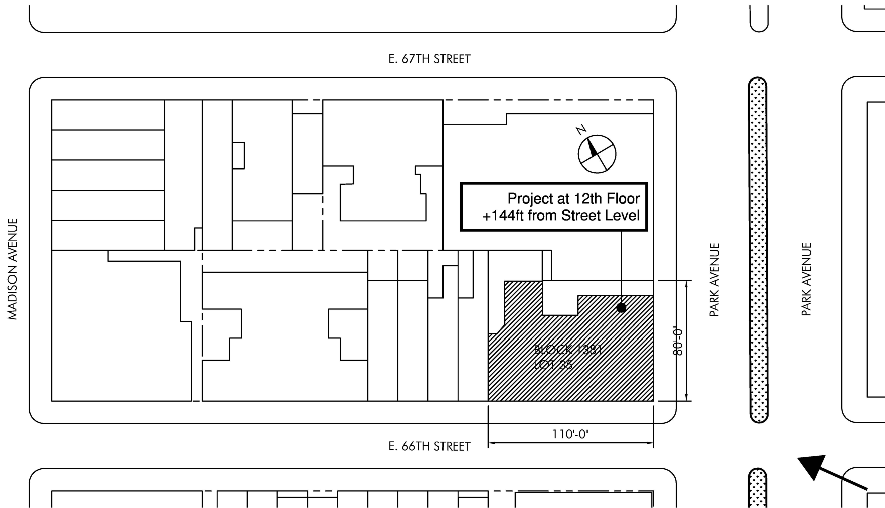
LOCATION PLAN
