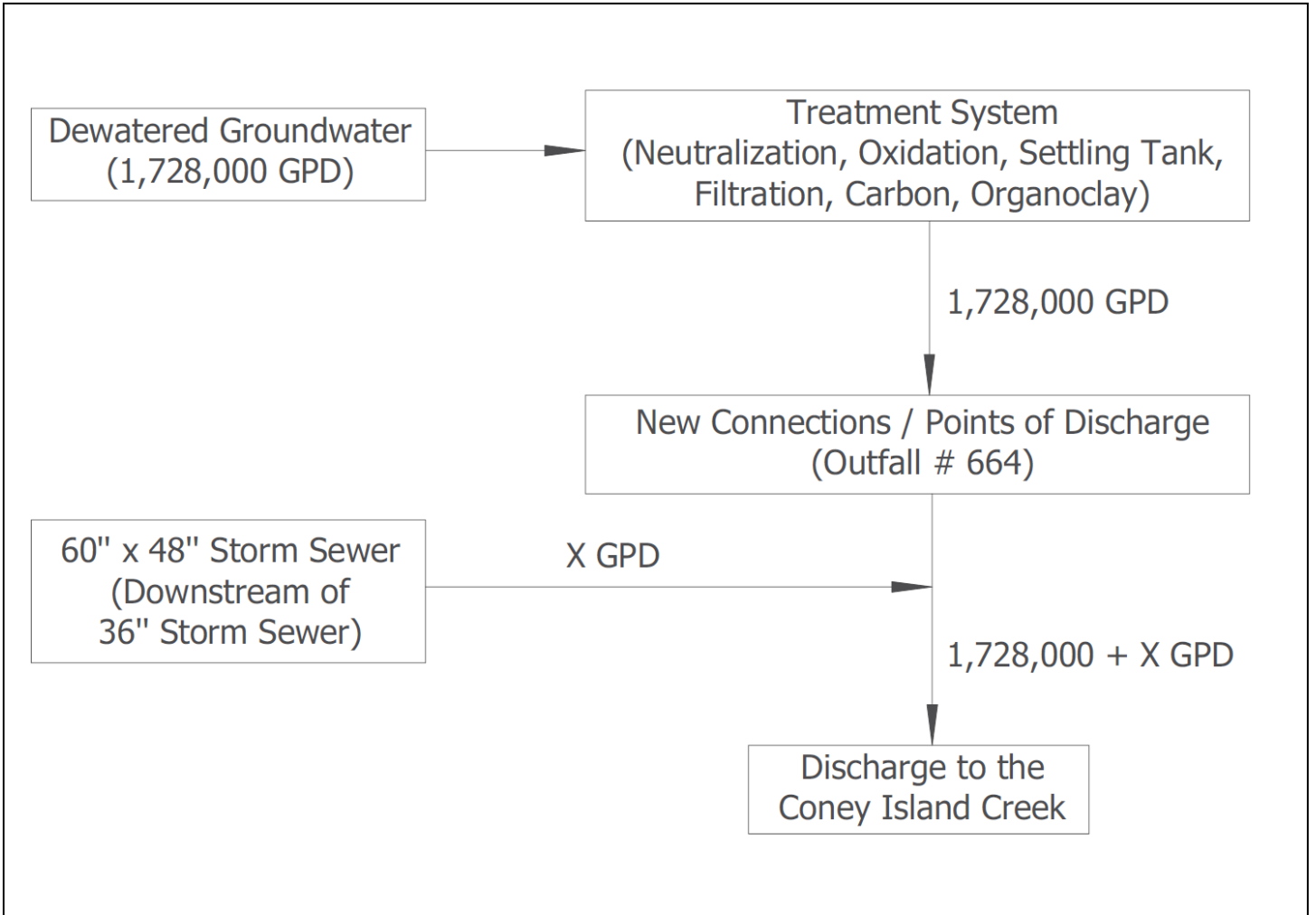
Schematic of Treatment System
