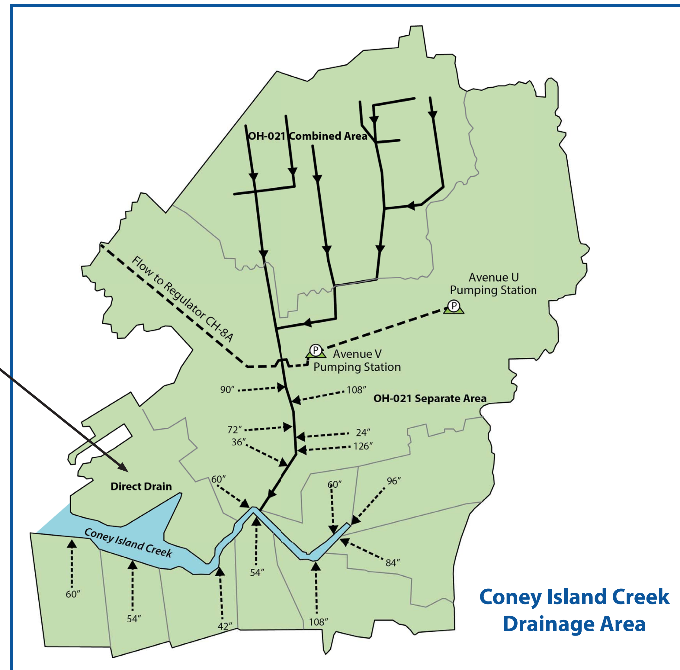
Coney Island Creek Model Grid
