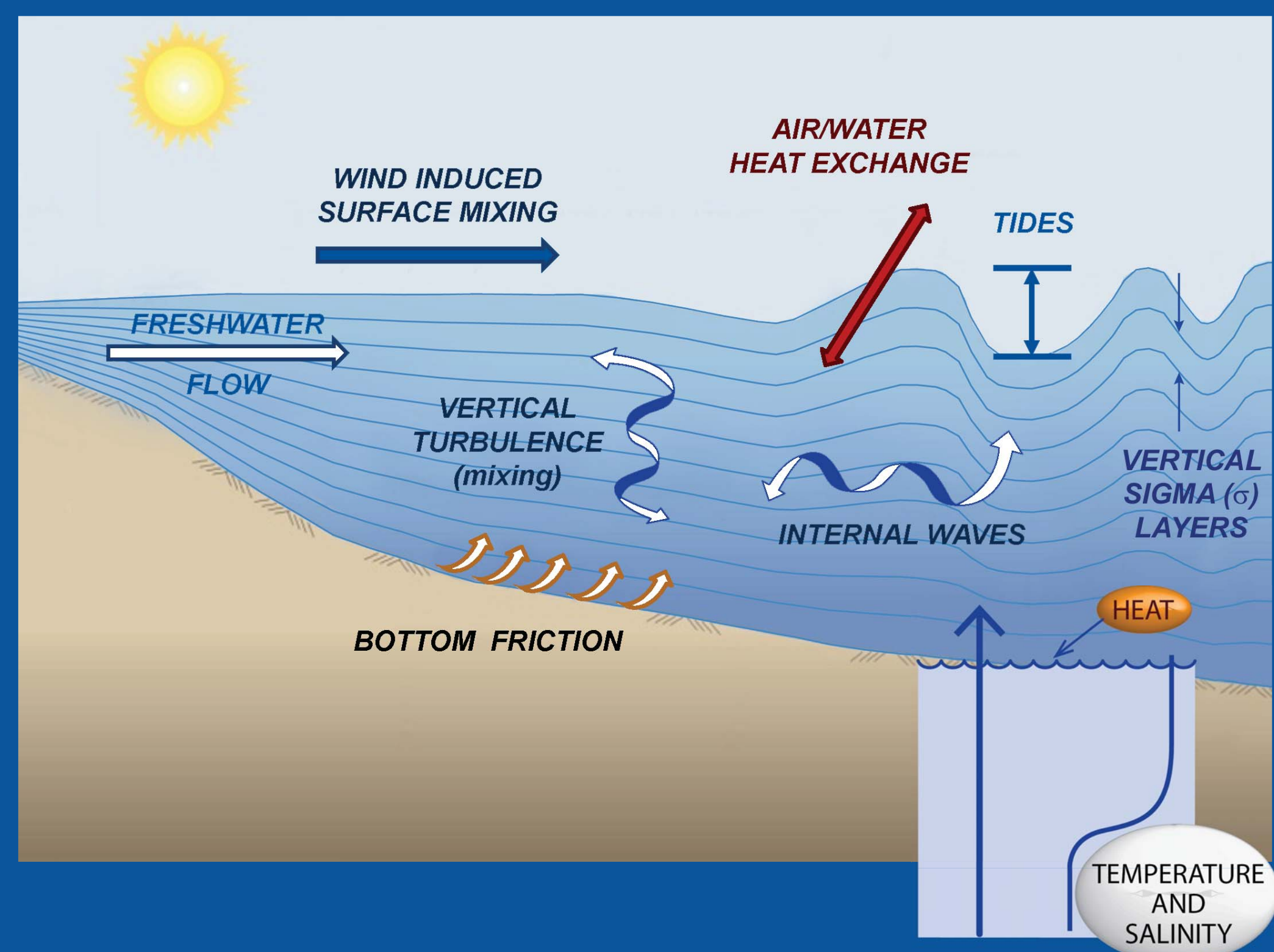
Hydrodynamic Model
