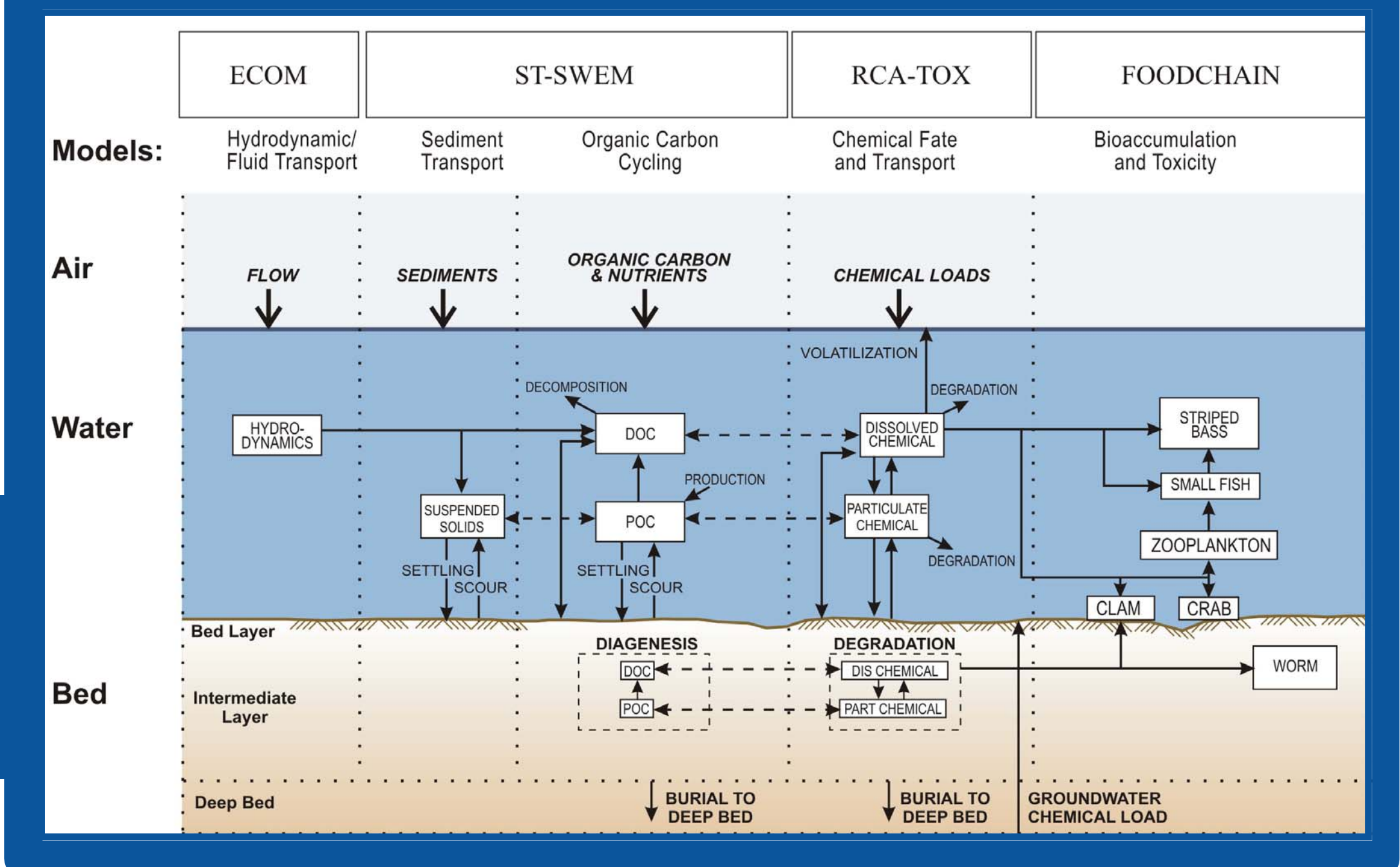
Sediment Transport and Toxics Model
