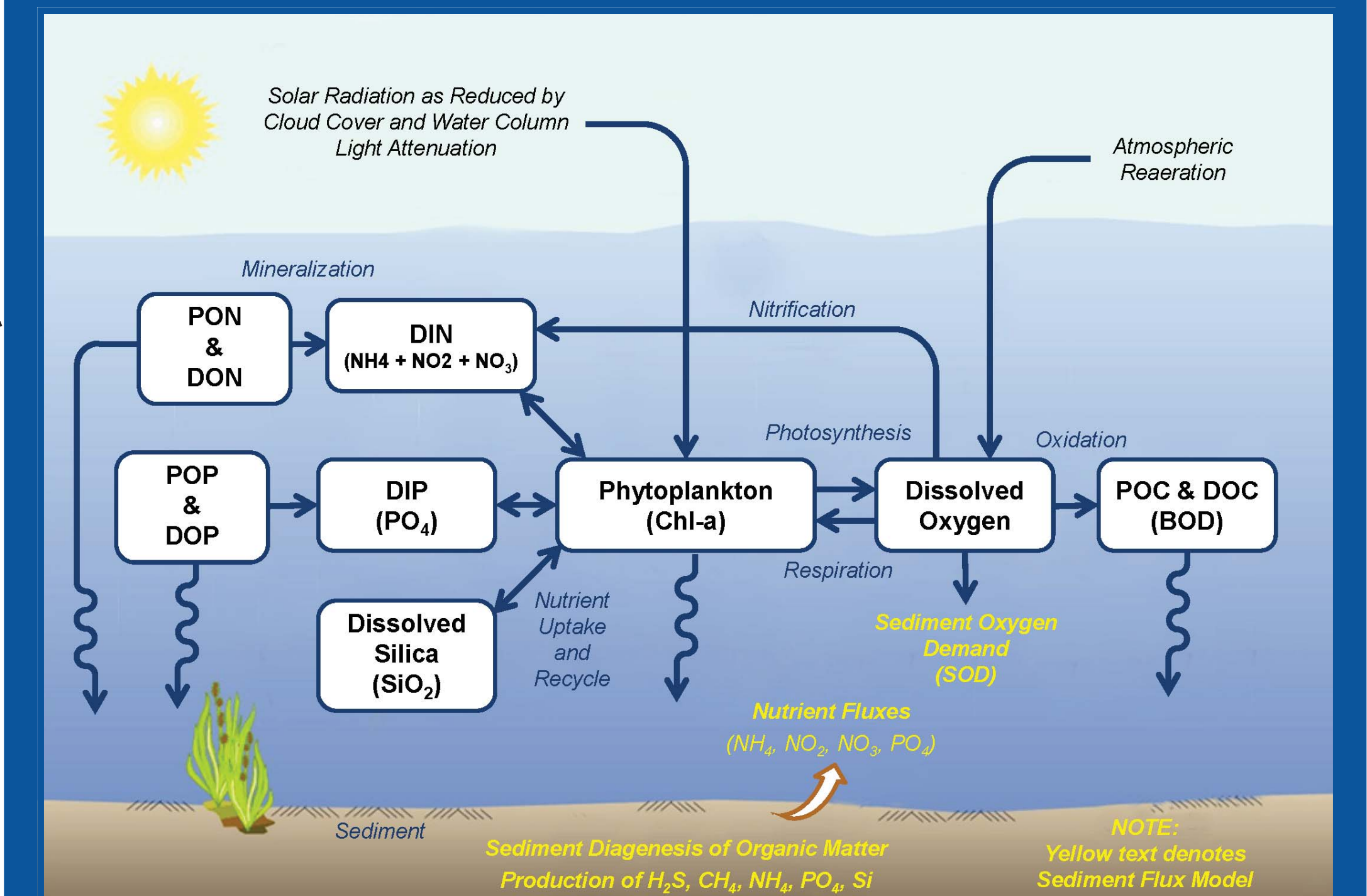
Eutrophication Model
