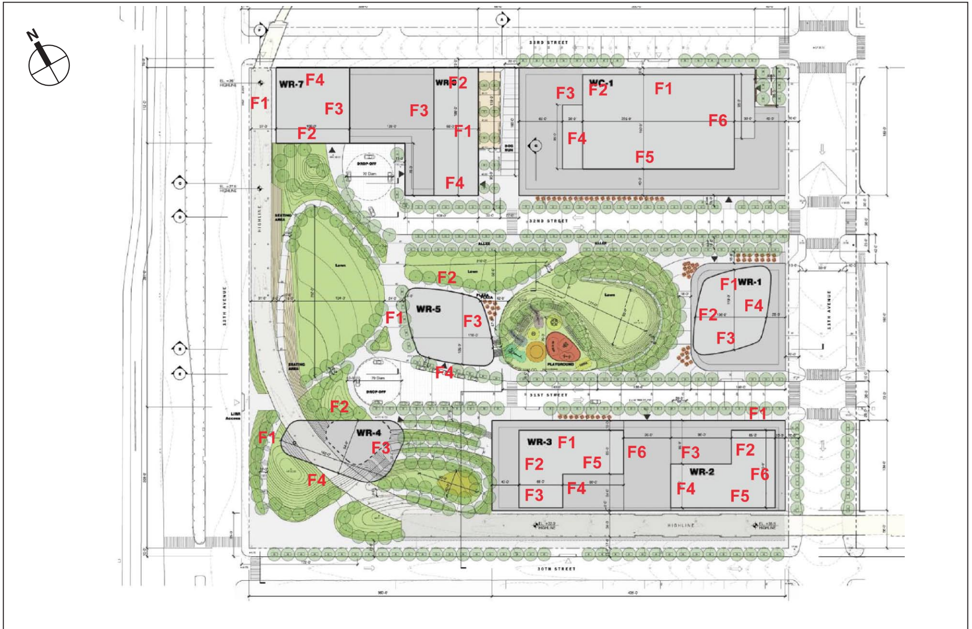
Window-Wall Noise Attenuation Requirements by Building Facade Figure 20-3
